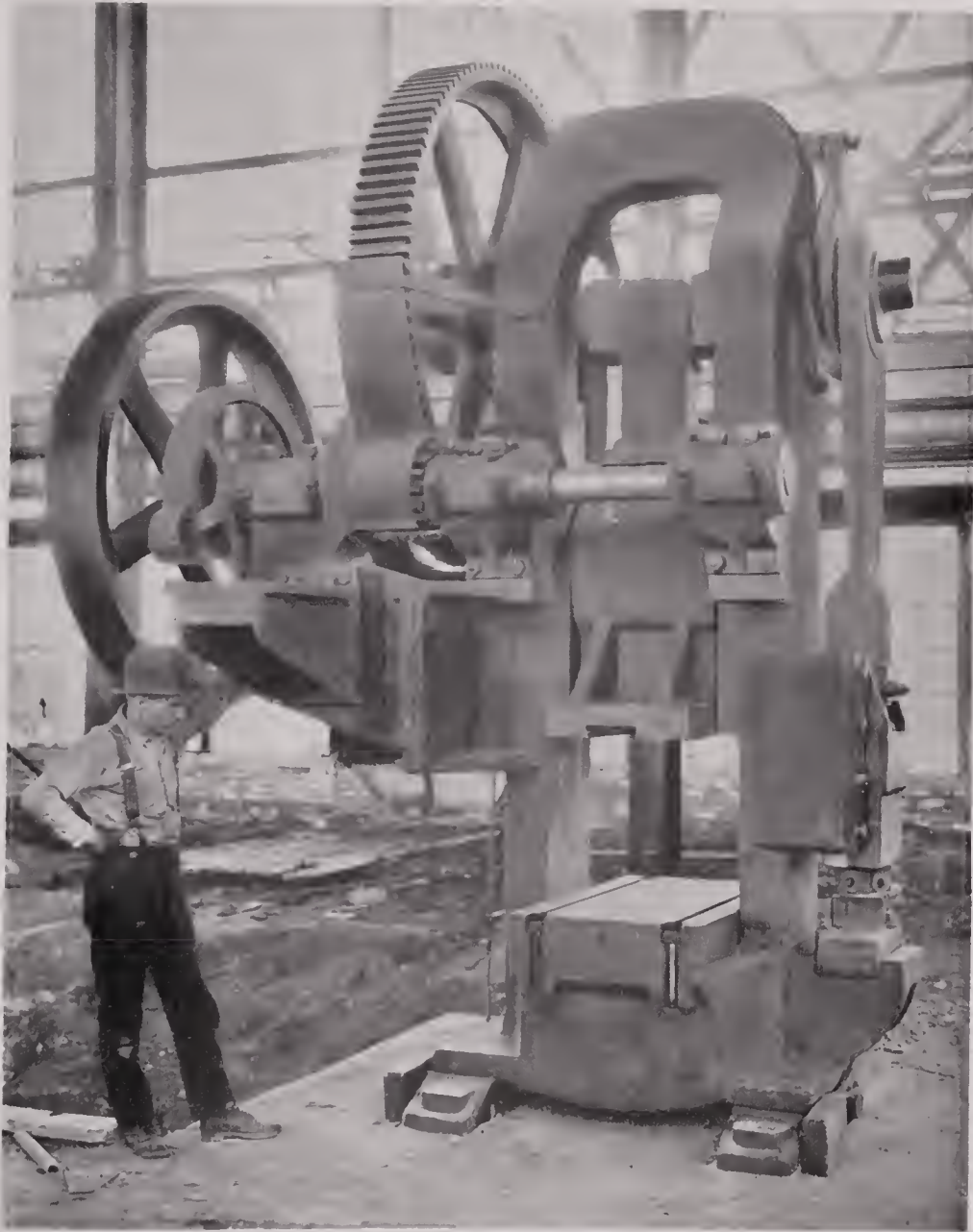
TOLEDO NO. 5S TRIMMING PRESS There Also Are Two of This Size Set Up
